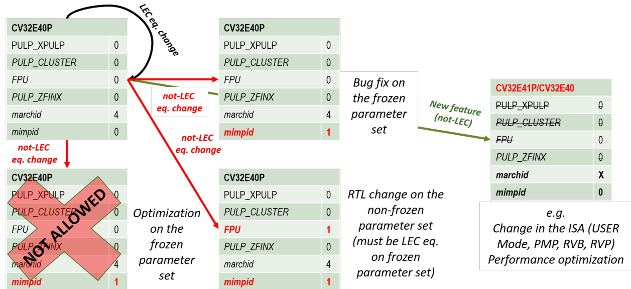
Figure 18.1: Versions control of CV32E40P
